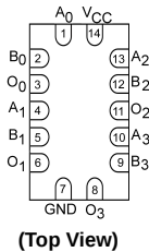
Pad Assignments for DQFN
