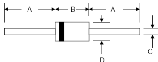
DO-41
