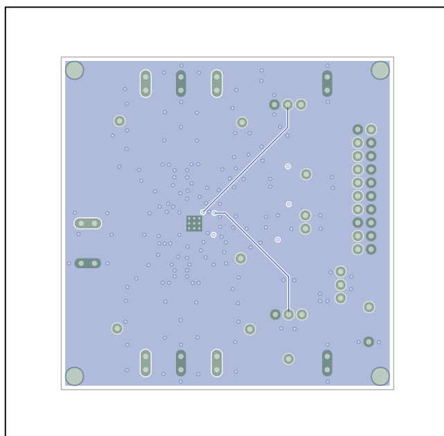
MAX20087 EV Kit PCB Layout—Bottom Copper
