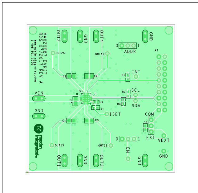
MAX20087 EV Kit Component Placement Guide—Top Copper and Silkscreen
