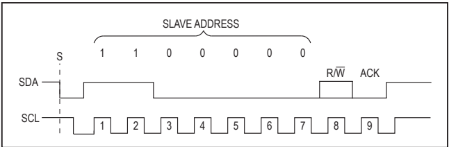
Figure 1. MAX2112 Slave Address Byte with ADDR Pin Connected to Ground
