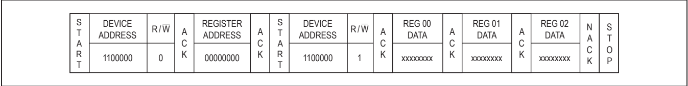
Figure 3. Example: Receive Data from Read Registers
