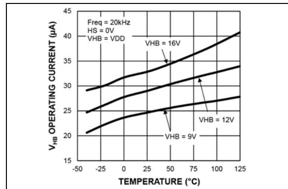
FIGURE 2-6: V_{HB} Operating Current vs. Temperature.
