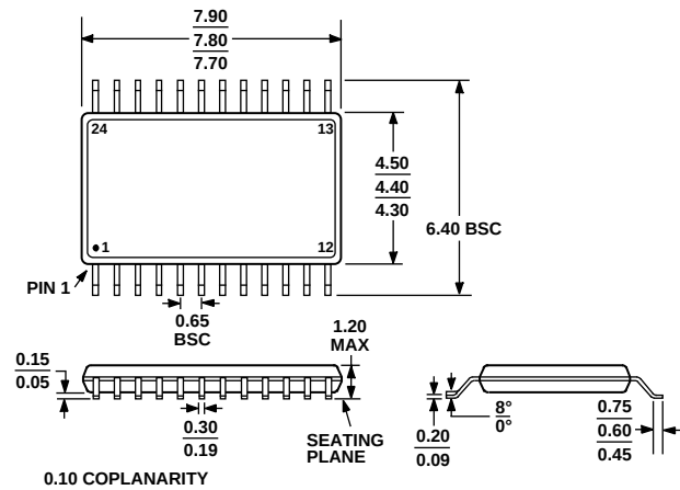
Figure 49. 24-Lead Thin Shrink Small Outline Package [TSSOP] (RU-24) Dimensions shown in millimeters
