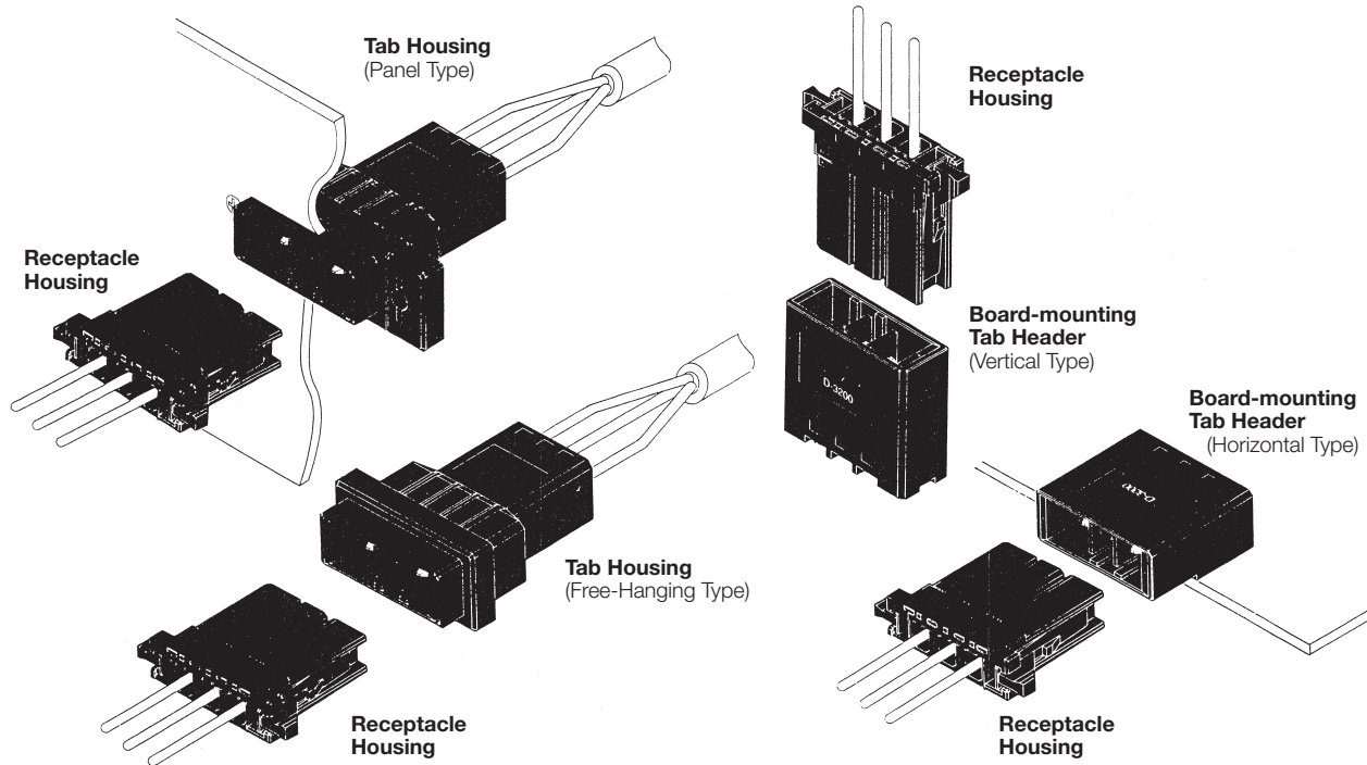
Receptacle Housing
