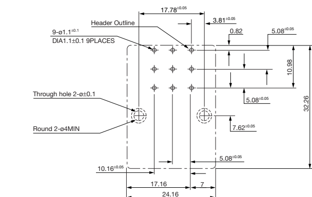
PC Board Layout Applicable Board Thickness: 1.6±0.1
