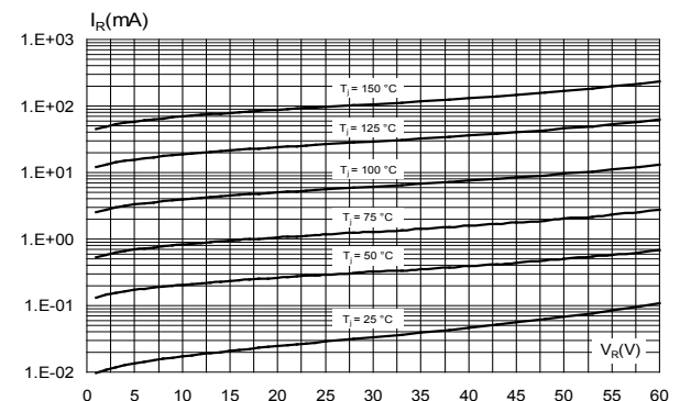
Figure 4. Reverse leakage current versus reverse voltage applied (typical values, per diode)
