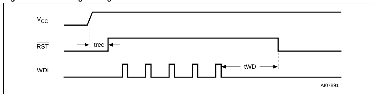
Figure 37. Watchdog Timing
