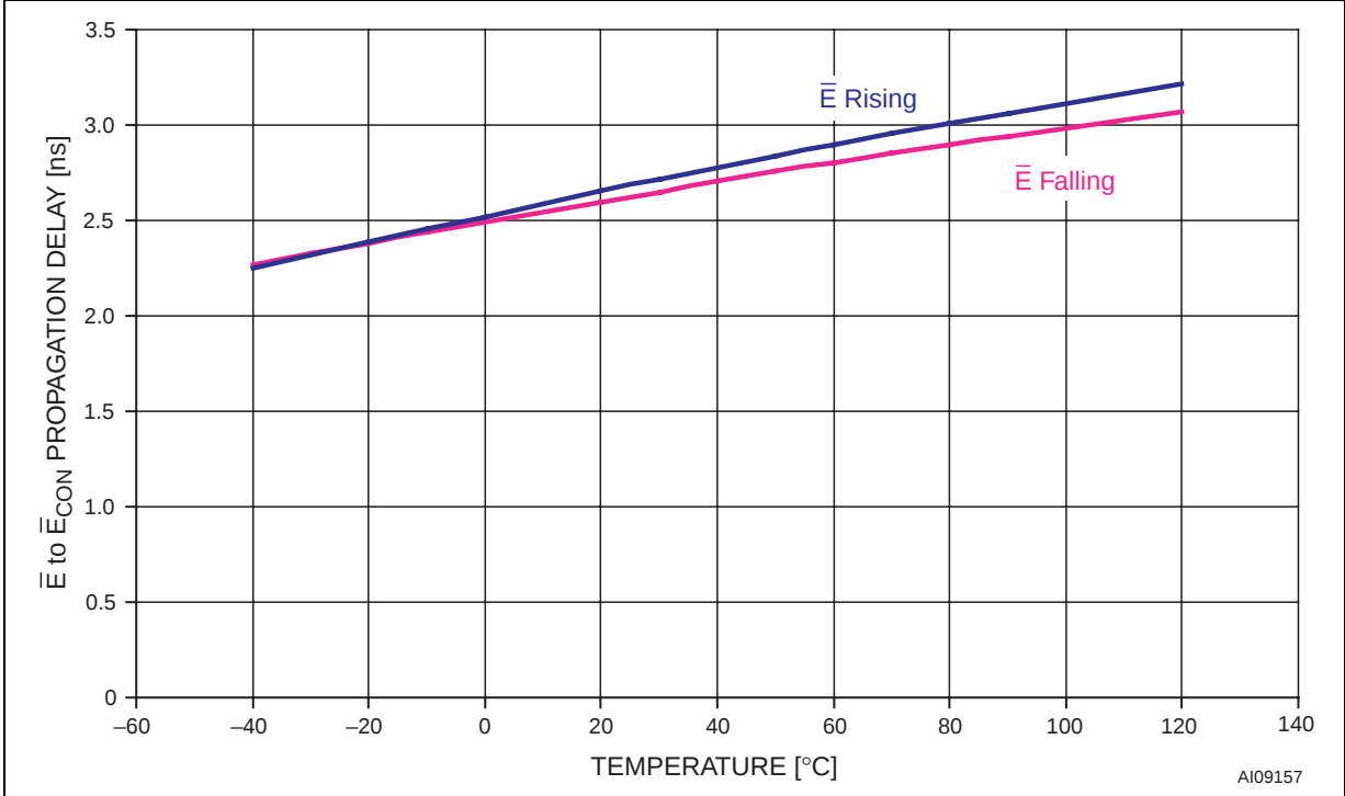
Figure 33. \bar{E} to \bar{E}_{\text{CON}} Propagation Delay vs. Temperature
