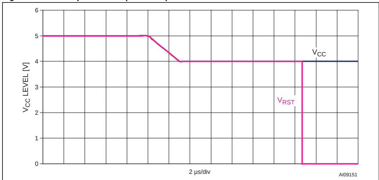
Figure 27. \overline{RST} Response Time (Assertion)
