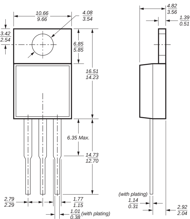
TO-220
