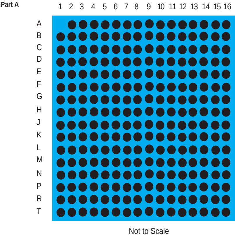
Figure 2. Pinout of the PC745, 255 PBGA Package as Viewed from the Top Surface
