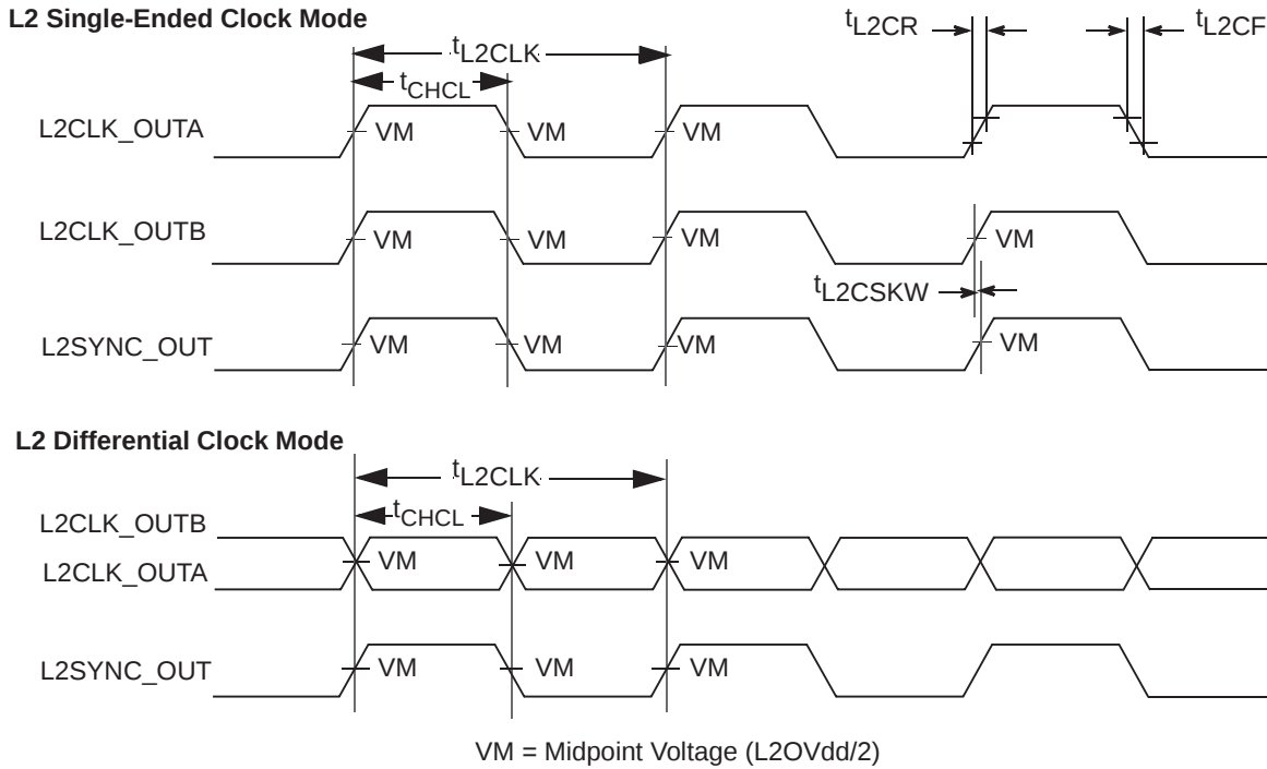
Figure 14. L2CLK_OUT Output Timing Diagram
