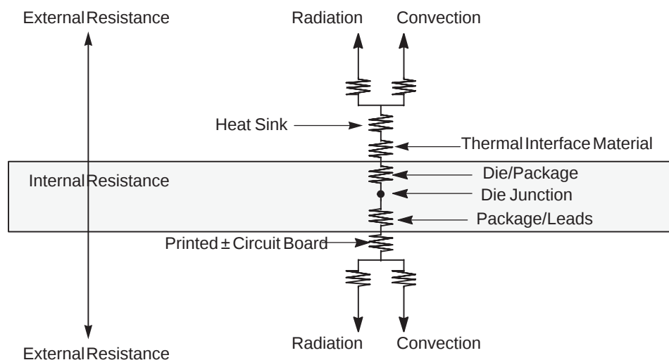
Figure 6. C4 Package with Head Sink Mounted to a Printed-circuit Board
