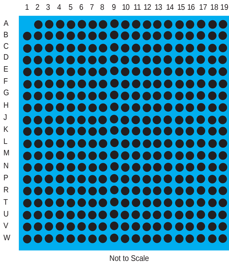
Figure 3. Pinout of the PC755, 360 PBGA, CBGA and CI-CGA Packages as Viewed from the Top Surface
