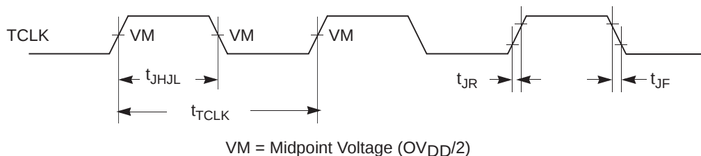
Figure 19. JTAG Clock Input Timing Diagram
