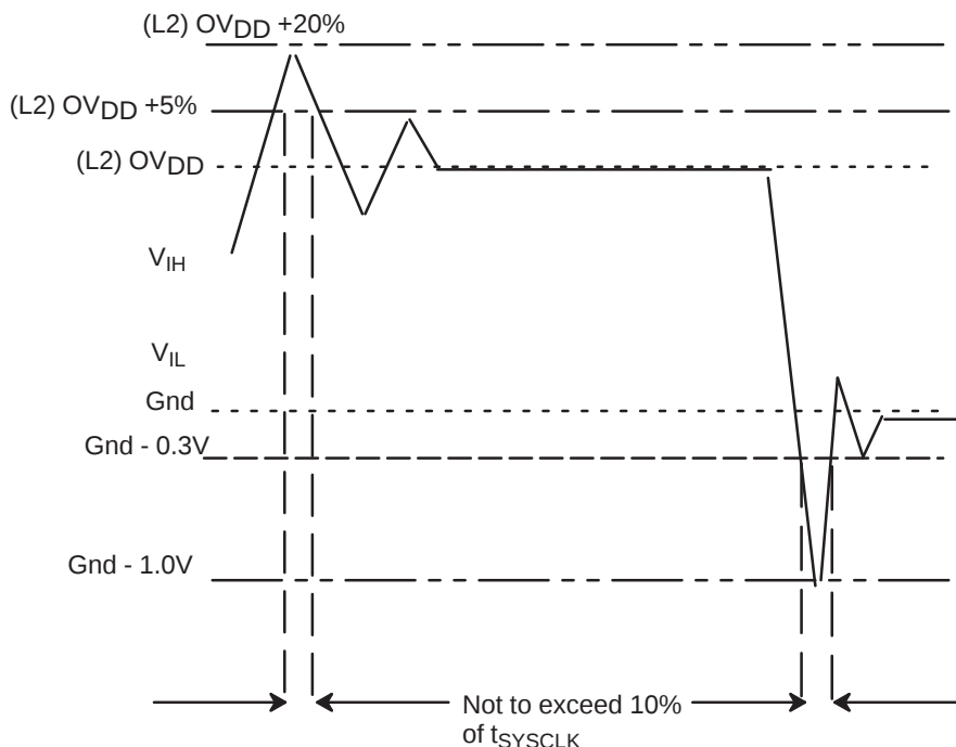
Figure 5. Overshoot/Undershoot Voltage
