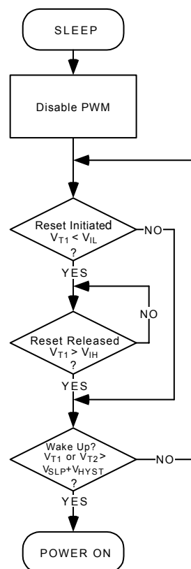
Figure 5. Sleep-Mode Behavior
