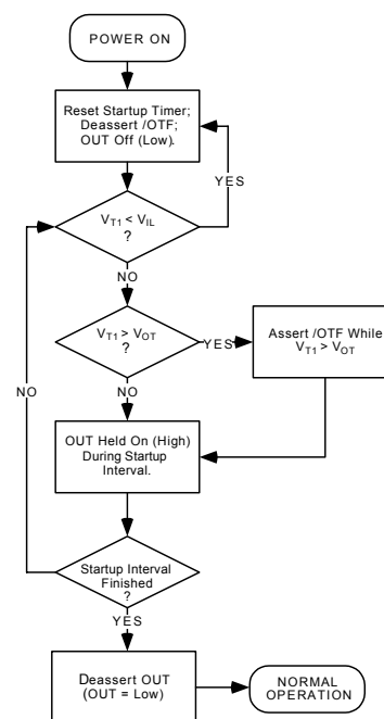
Figure 3. Power-Up Behavior
