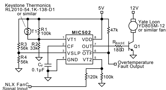
Figure 7. Typical 5V V_{DD} Application Circuit
