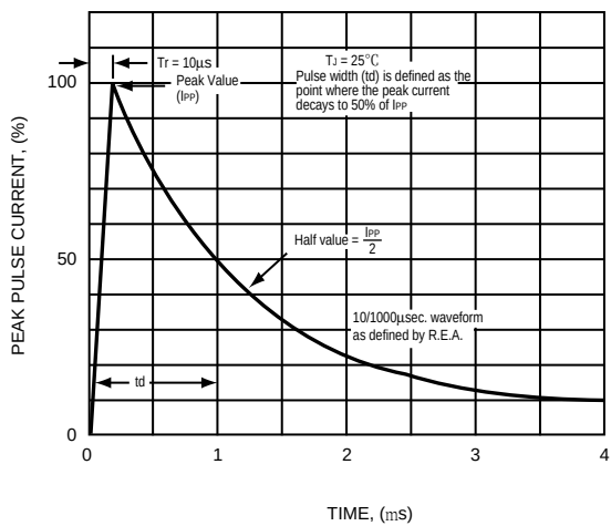
FIG. 4 - PULSE WAVEFORM
