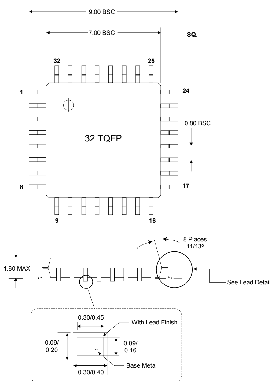
Figure 2. Package information
