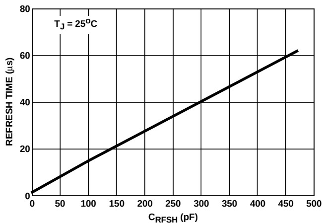
FIGURE 14. REFRESH TIME
