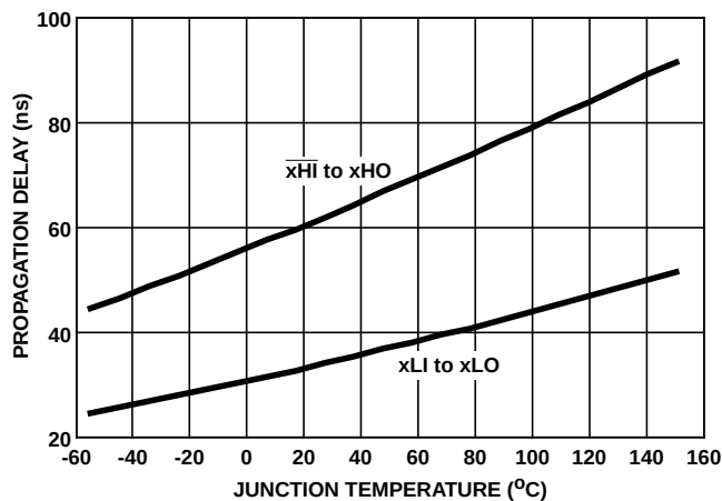
FIGURE 12. PROPAGATION DELAY
