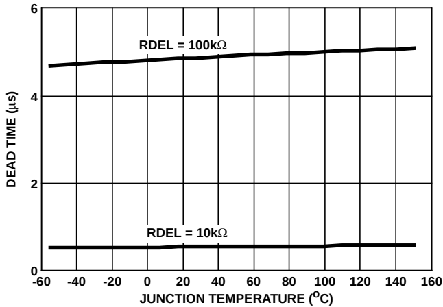
FIGURE 15. DEAD TIME
