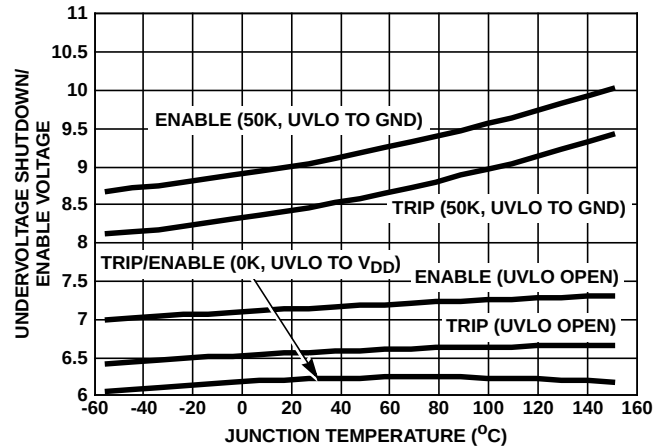
FIGURE 16. UNDERVOLTAGE THRESHOLD
