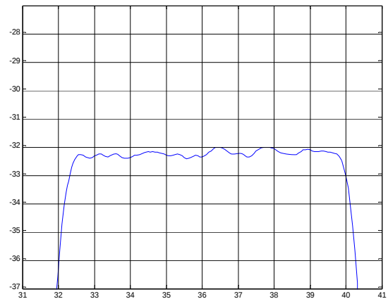
Phase Linearity ( f_0 \pm 3.5 MHz)
