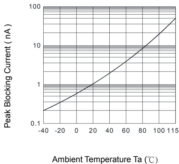
Fig.8 Leakage with LED off vs. Ambient Temperature
