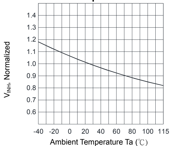
Fig.6 Inhibit Voltage V_{INH} vs. Ambient Temperature
