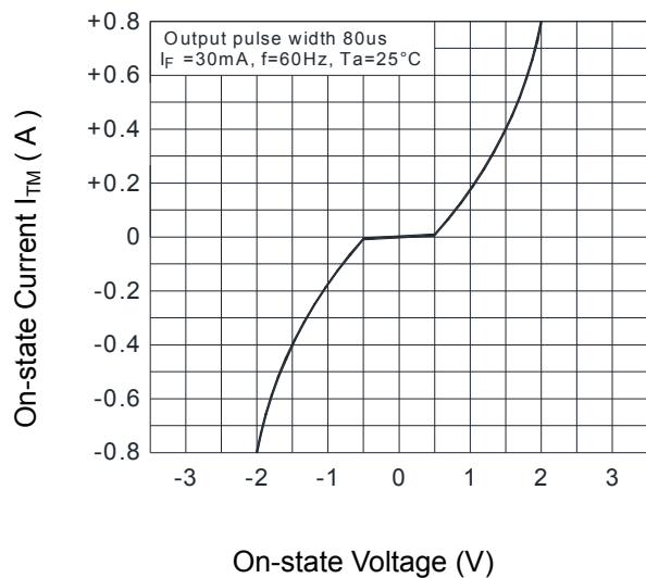
Fig.7 On-state Characteristics
