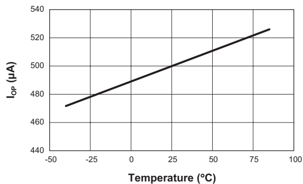
Operating Current vs. Temperature ( V_{IN} = 5.0V ; R_{SET} = 8.06k\Omega )
