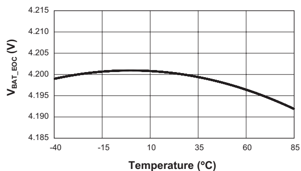
End of Charge Voltage Regulation vs. Temperature
