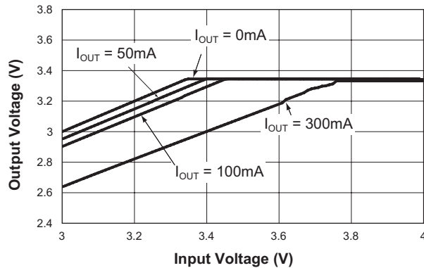
Dropout Characteristics
