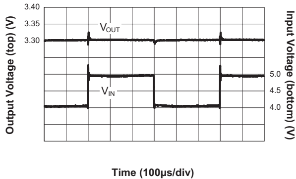
Line Transient Response ( I_{OUT} = 300\text{mA} )
