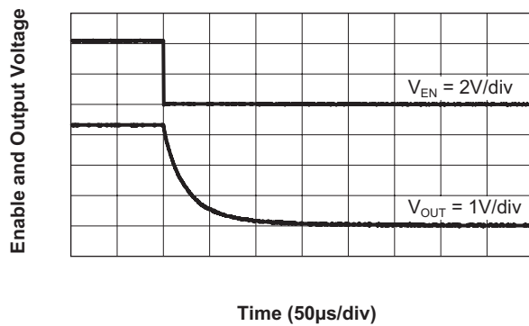
Turn-Off Response Time ( V_{IN} = 4.2\text{V} ; I_{OUT} = 300\text{mA} )
