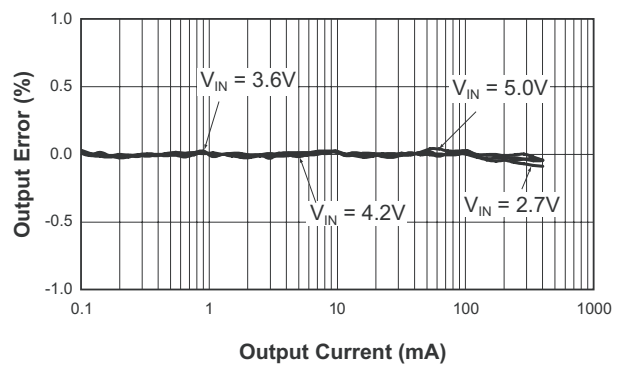
DC Regulation ( V_{OUT} = 1.2V ; L = 1.5\mu H )
