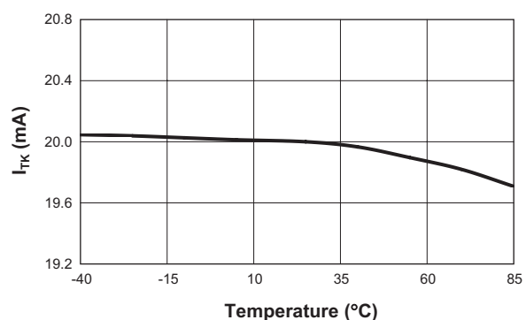
Preconditioning Charge Current vs. Temperature
