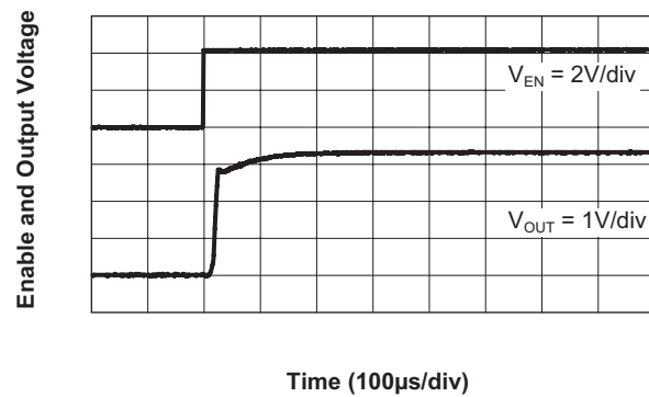
Turn-On Time From Enable ( V_{IN} = 4.2\text{V} ; I_{OUT} = 300\text{mA} )
