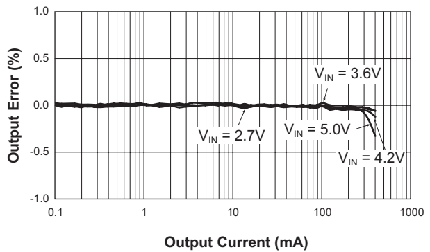
DC Regulation ( V_{OUT} = 1.8V ; L = 3.3\mu H )
