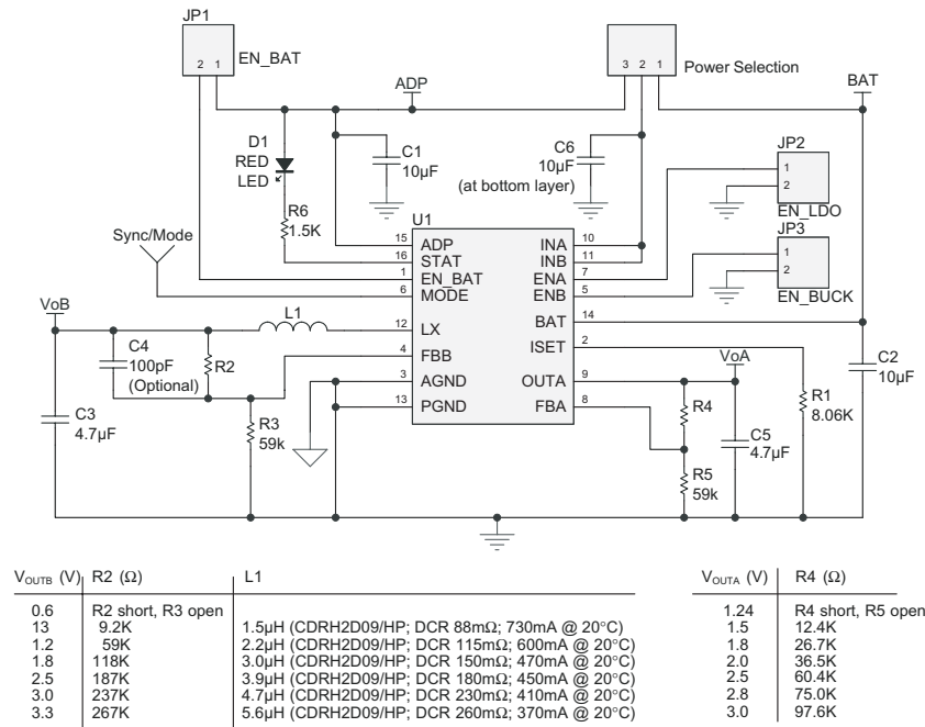
Figure 5: AAT2552 Evaluation Board Schematic.
