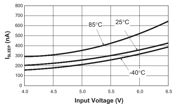
Sleep Mode Current vs. Input Voltage ( R_{SET} = 8.06k\Omega )
