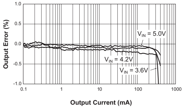
DC Regulation ( V_{OUT} = 3.3V ; L = 5.6\mu H )
