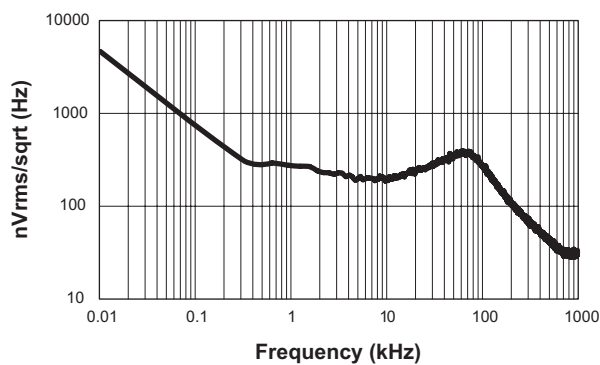
LDO Output Noise ( C_{OUT} = 4.7\mu\text{F} ; I_{OUT} = 10\text{mA} ; R_{LOAD} = 330 ; 98.33µVrms)
