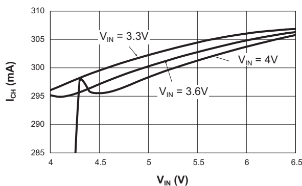
Constant Charging Current vs. Input Voltage
