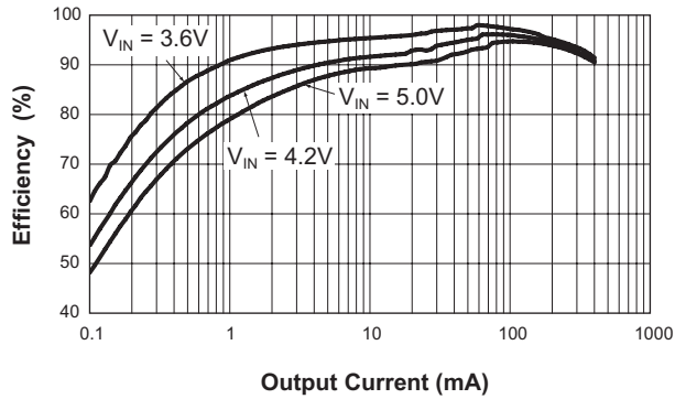
Efficiency vs. Load ( V_{OUT} = 3.3V ; L = 5.6\mu H )
