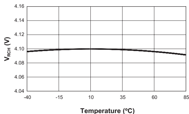
Recharging Threshold Voltage vs. Temperature
