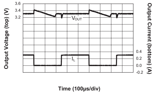
Load Transient Response (1mA to 300mA; V_{IN} = 5.0\text{V} ; V_{OUT} = 3.3\text{V} )
