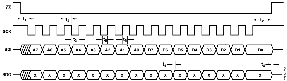
Figure 3. SPI Write Timing Diagram
