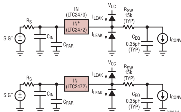
Figure 16. LTC2470/LTC2472 Input Drive Equivalent Circuit
