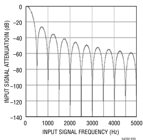
Figure 20. LTC2472 Input Signal Attenuation vs Frequency (208sps Mode)
