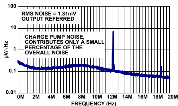
FIGURE 24. NOISE SPECTRUM
