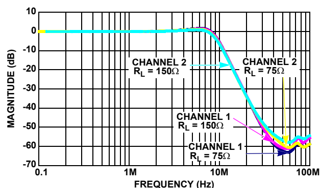
FIGURE 1. BANDWIDTH vs FREQUENCY
