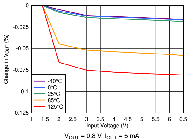
图 7-29. Line Regulation
