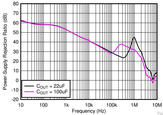
图 7-7. PSRR vs Frequency and C_{OUT}
