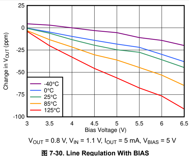
图 7-30. Line Regulation With BIAS
