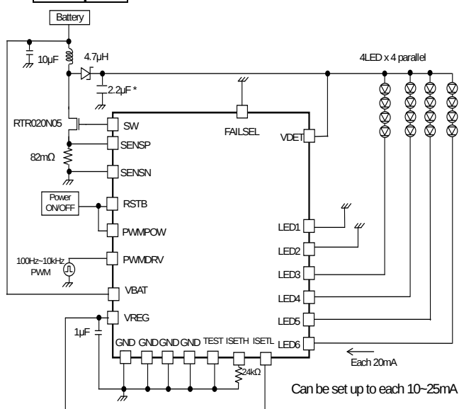
Figure 56. 4 series \times 4 parallel, LED current 20mA setting Current driver PWM application
