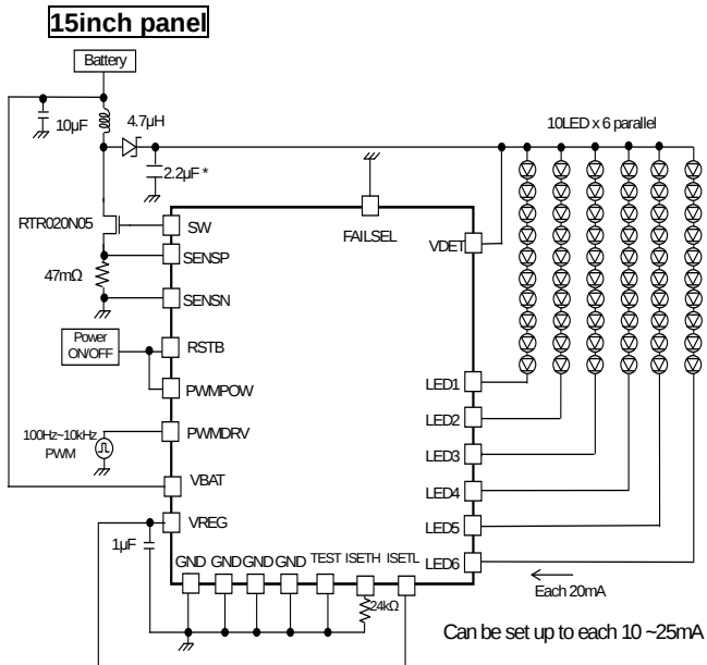
Figure 45. 10 series \times 6 parallel, LED current 20mA setting Current driver PWM application
