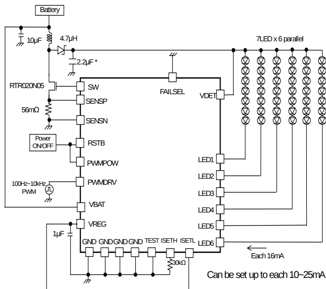
Figure 48. 7 series \times 6 parallel, LED current 16mA setting Current driver PWM application
