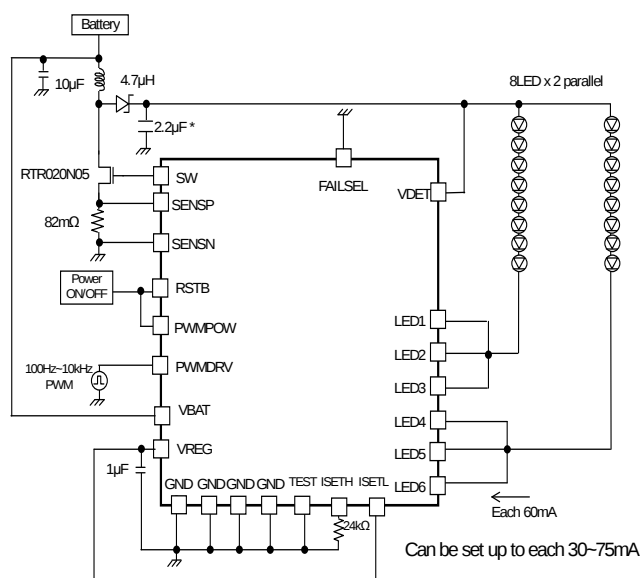
Figure 57. 8 series \times 2 parallel, LED current 60mA setting Current driver PWM application
