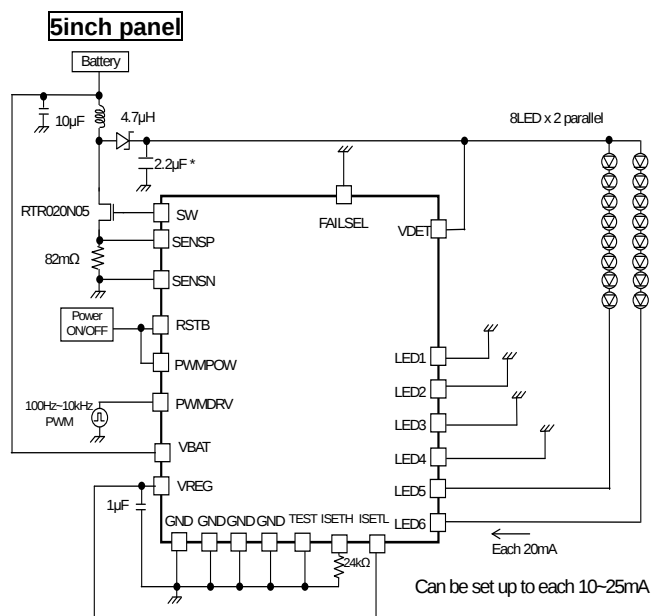
Figure 54. 8 series \times 2 parallel, LED current 20mA setting Current driver PWM application
