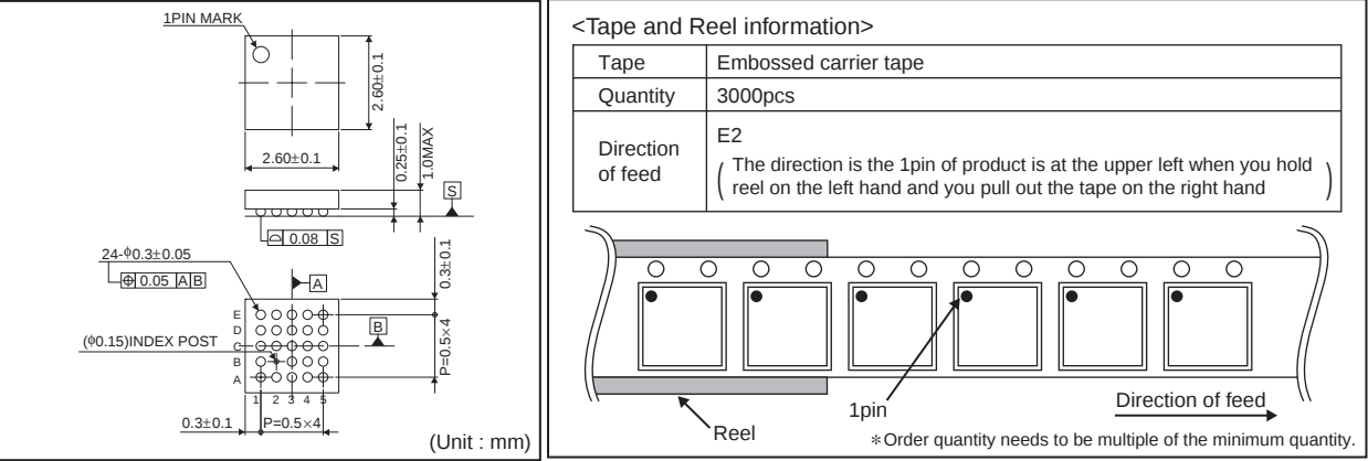
Figure 64 VCSP85H2 (BD6581GU)
