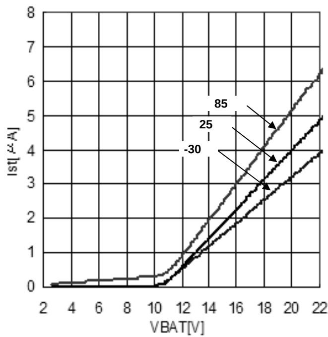
Figure 5. Quiescent current vs VBAT
