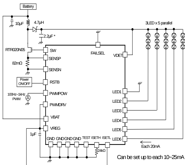
Figure 58. 3 series \times 5 parallel, LED current 20mA setting Power control PWM application
