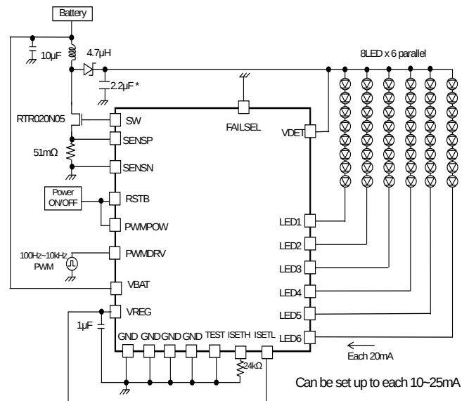
Figure 47. 8 series \times 6 parallel, LED current 20mA setting Current driver PWM application
