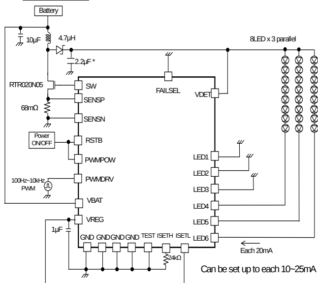
Figure 50. 8 series \times 3 parallel, LED current 20mA setting Current driver PWM application
