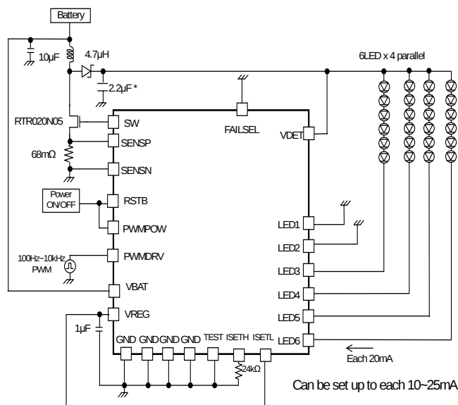
Figure 51. 6 series \times 4 parallel, LED current 20mA setting Current driver PWM application
