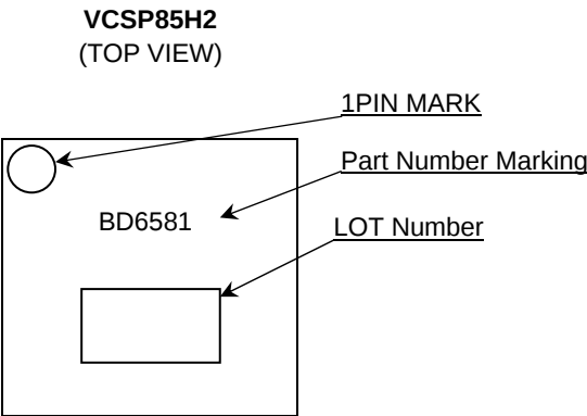
Figure 63 Marking Diagram
