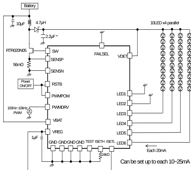
Figure 49. 10 series \times 4 parallel, LED current 20mA setting Current driver PWM application
