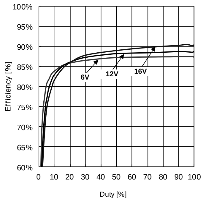
Figure 9. Efficiency vs PWMDRV-HI Duty I SETH =24k \Omega , PWM=200Hz
