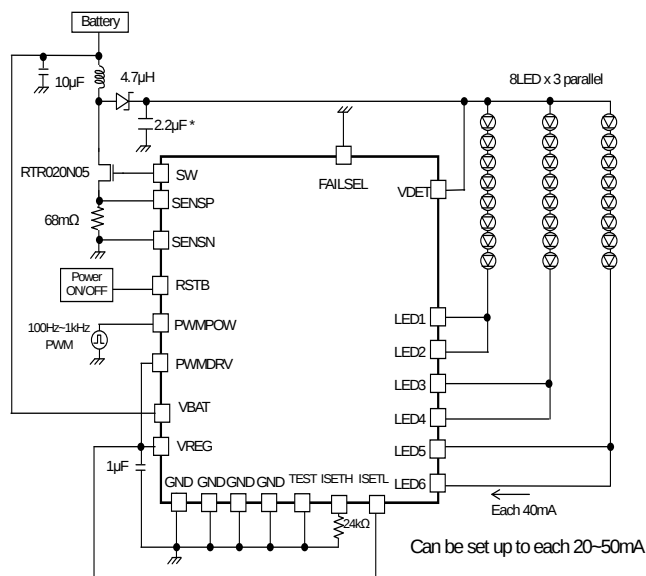
Figure 53. 8 series \times 3 parallel, LED current 40mA setting Power control PWM application
