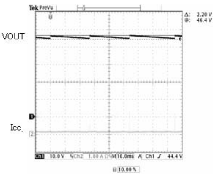
Figure 25. VOUT@OVP (LED OPEN)
