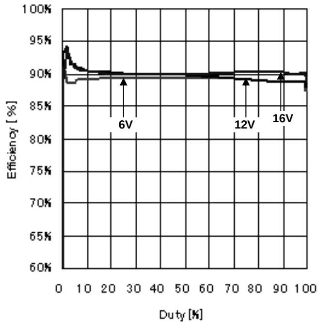
Figure 8. Efficiency vs PWMPOW-HI Duty I SETH =24k \Omega , PWM=200Hz
