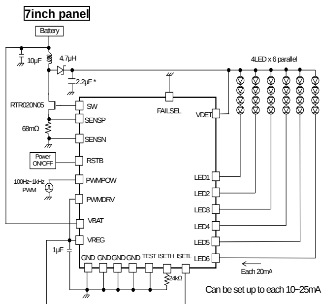
Figure 52. 4 series \times 6 parallel, LED current 20mA setting Power control PWM application
