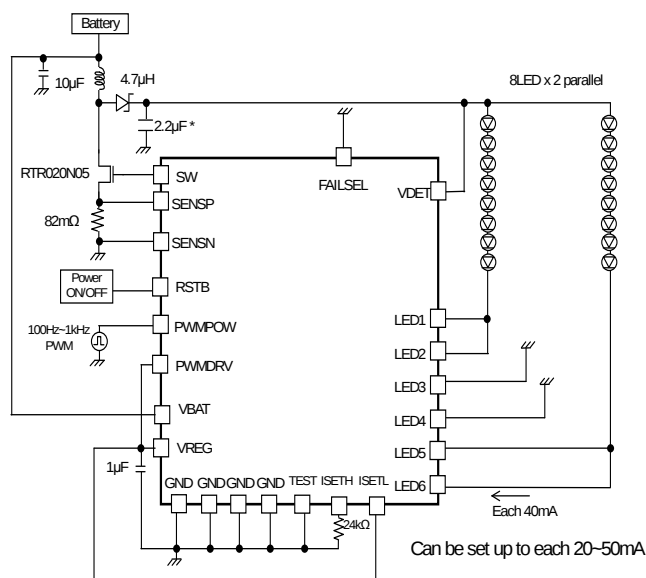
Figure 55. 8 series \times 2 parallel, LED current 40mA setting Power control PWM application
