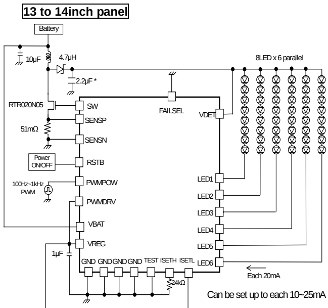
Figure 46. 8 series \times 6 parallel, LED current 20mA setting Power control PWM application
