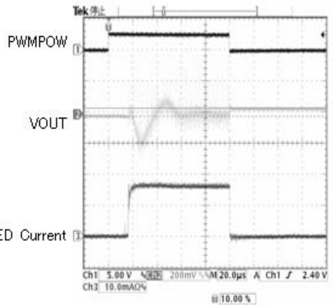
Figure 21. VOUT response Power Control PWM (PWMPOW)
