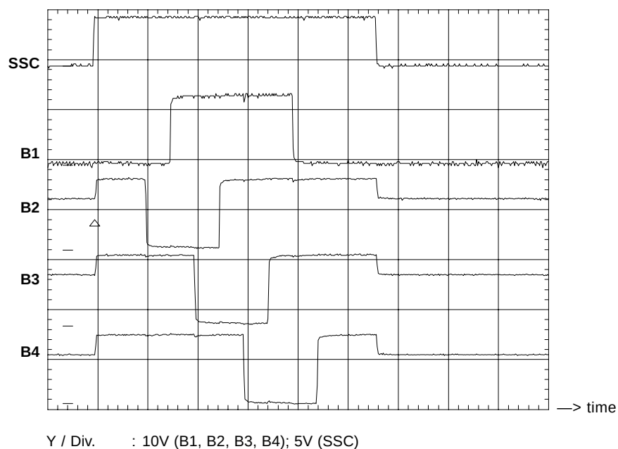
Figure 5 - Vertical readout
