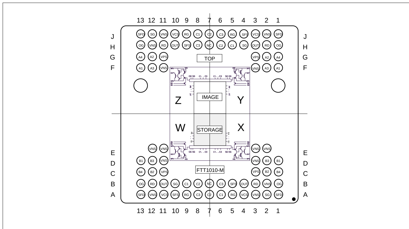
Figure 13 - FTT1010-M pin configuration (top view)
