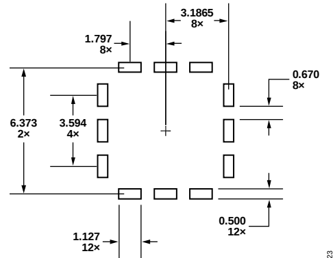
Figure 5. Second-Level Assembly Pad Layout
