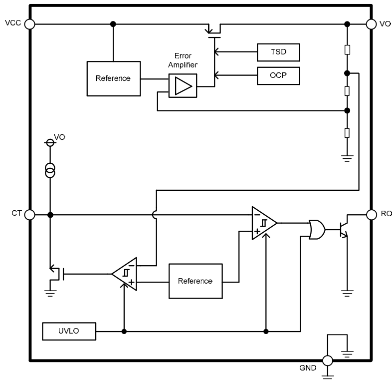
Figure 4. Block Diagram
