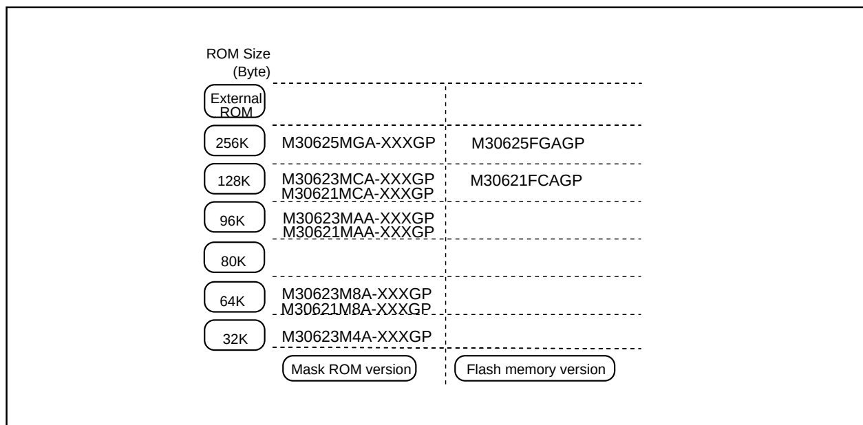
Figure 1.1.3. ROM expansion
