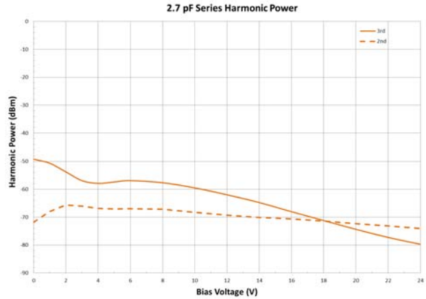
Figure 3. Harmonic Power*
