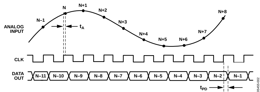
Figure 2. Timing Diagram
