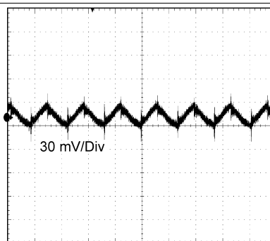
TIME (2 \mu\text{s/Div} ) 12 V_{IN} , 5 V_{OUT} at Full Load, BW = 250 MHz
