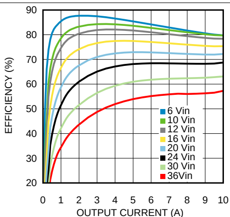
Figure 7. Efficiency 1.8-V Output at 25°C
