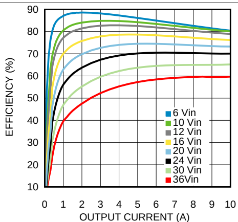
Figure 19. Efficiency 2.5-V Output at 85°C
