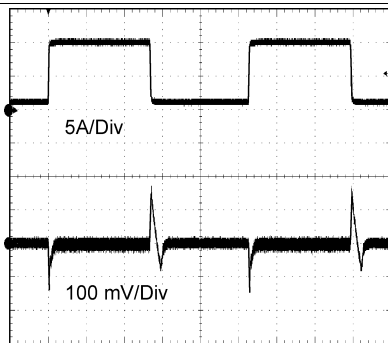
Figure 39. Transient Response
