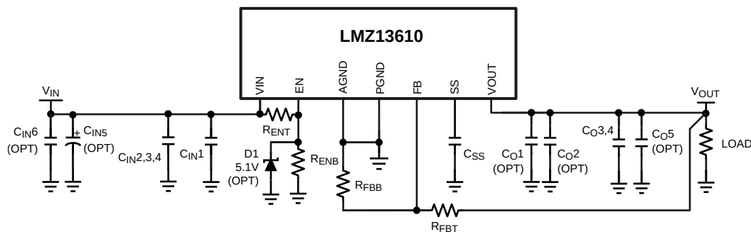
Figure 47. Typical Application Schematic
