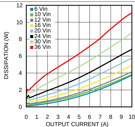
Figure 10. Dissipation 1.5-V Output at 25°C
