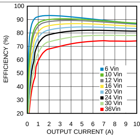
Figure 15. Efficiency 5-V Output at 85°C
