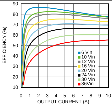
Figure 21. Efficiency 1.8-V Output at 85°C
