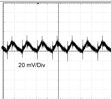
TIME (2 \mu\text{s/Div} ) 12 V_{IN} , 3.3 V_{OUT} at Full Load, BW = 250 MHz
