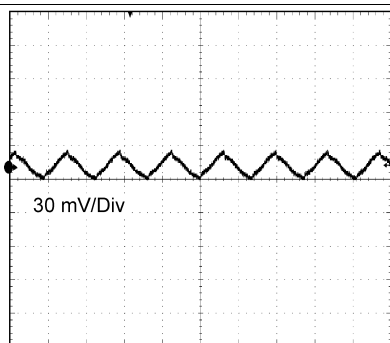
TIME (2 \mu\text{s/Div} ) 12 V_{IN} , 5 V_{OUT} at Full Load, BW = 20 MHz
