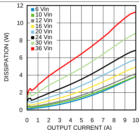
Figure 8. Dissipation 1.8-V Output at 25°C
