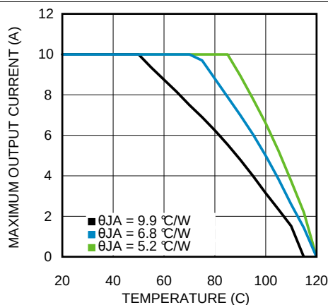
Figure 31. Thermal Derating
