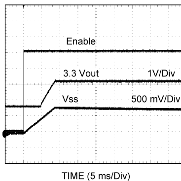
Figure 45. Prebiased Start-Up
