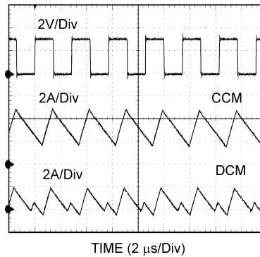
Figure 46. CCM and DCM Operating Modes
