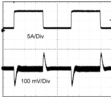
Figure 37. Output Ripple
