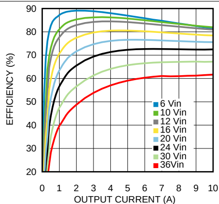
Figure 7. Efficiency 1.8-V Output at 25°C
