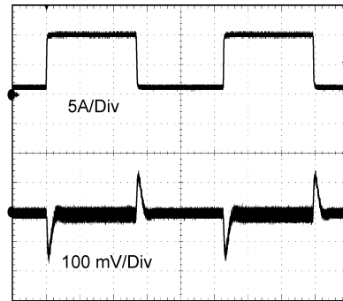
Figure 38. Output Ripple
