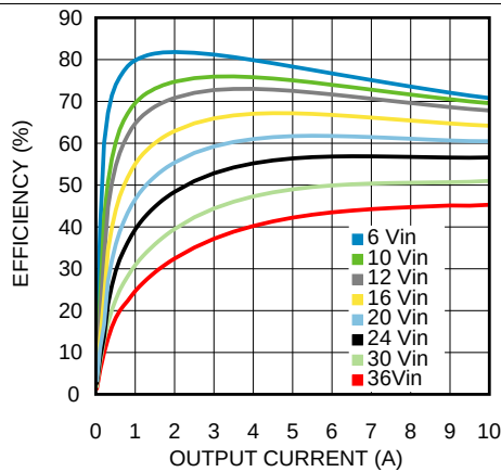
Figure 25. Efficiency 1.2-V Output at 85°C
