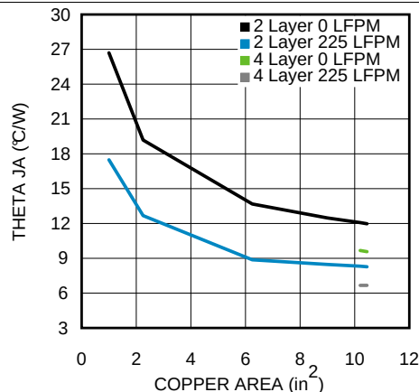
Figure 32. \theta_{JA} vs Copper Heat Sinking Area
