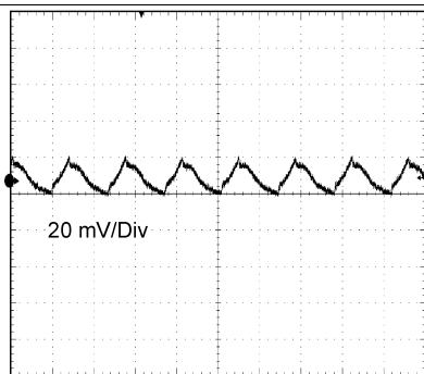
TIME (2 \mu\text{s/Div} ) 12 V_{IN} , 3.3 V_{OUT} at Full Load, BW = 20 MHz
