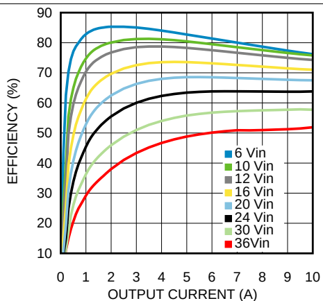
Figure 9. Efficiency 1.5-V Output at 25°C
