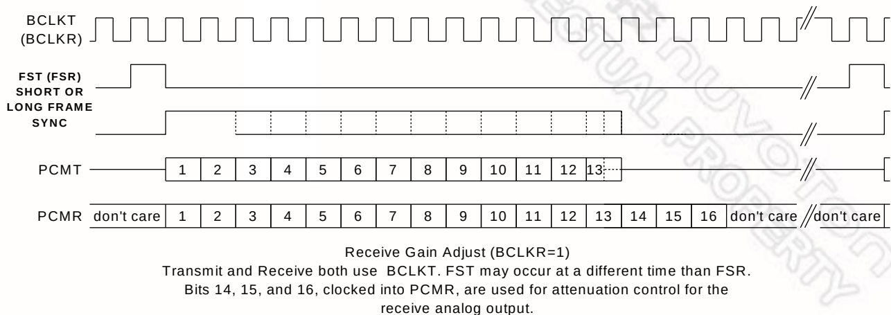
FIGURE 7.7: RECEIVE GAIN ADJUST TIMING MODE
