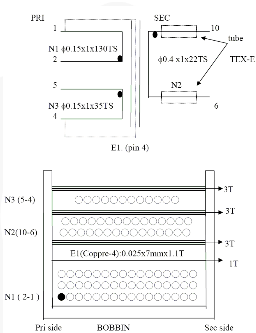
Figure 32. Transformer Diagram
