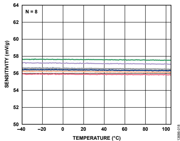
Figure 18. X-Axis Sensitivity vs. Temperature, V_S = 3\text{ V}
