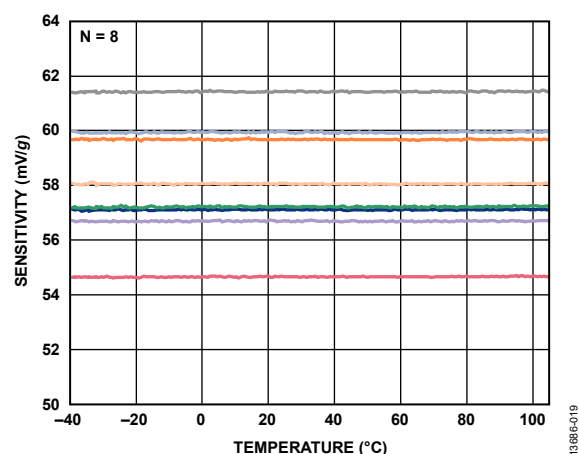
Figure 19. Y-Axis Sensitivity vs. Temperature, V_S = 3\text{ V}
