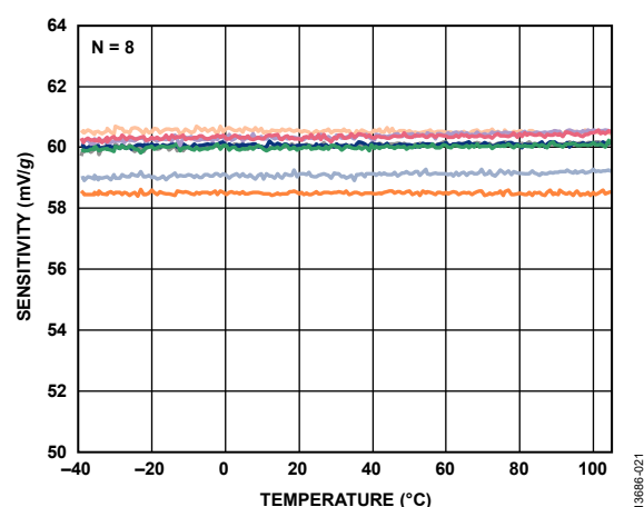
Figure 20. Z-Axis Sensitivity vs. Temperature, V_S = 3\text{ V}
