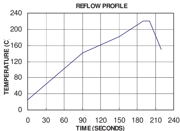
Figure 15 VPOL16A-12-SMT Reflow Profile
