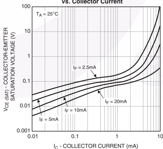
Fig. 6 Collector-Emitter Saturation Voltage vs. Collector Current
