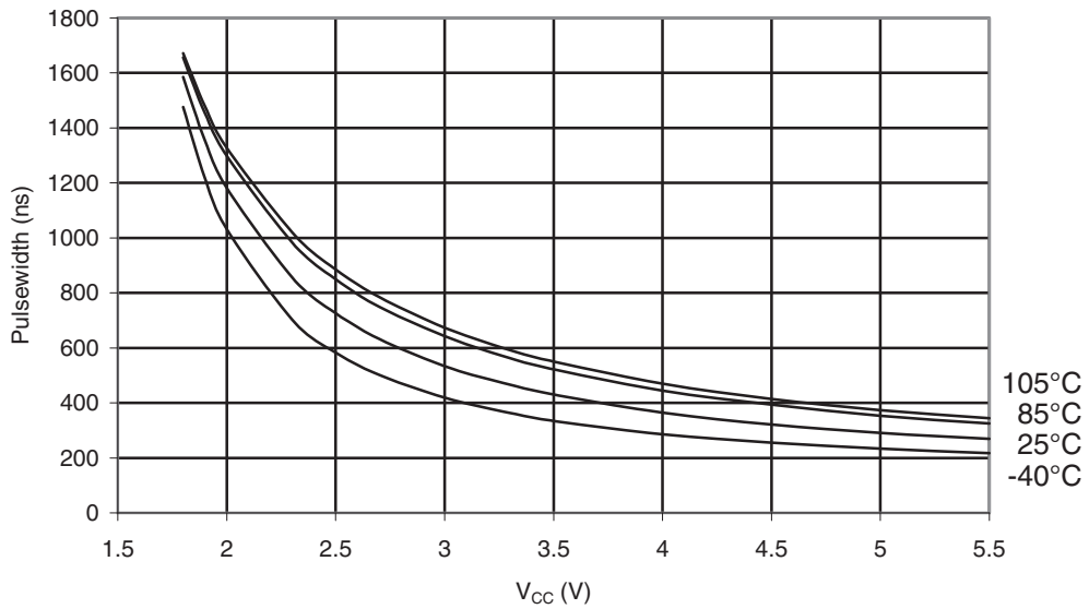
Figure 35-47. ATmega328P: Minimum Reset Pulse Width vs. Vcc
