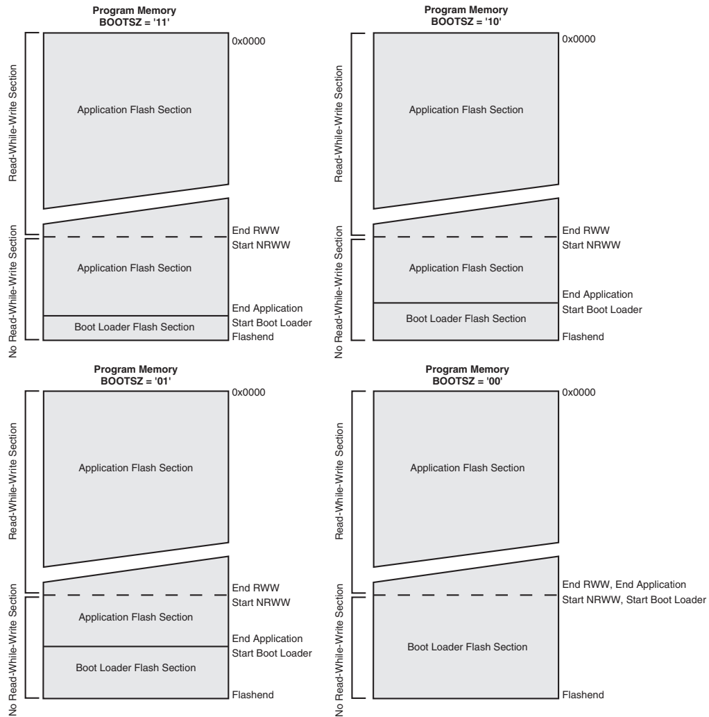
Figure 27-2. Memory Sections
