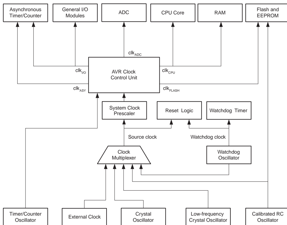
Figure 9-1. Clock Distribution
