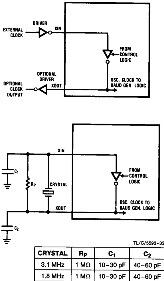
FIGURE 2. Typical Crystal Oscillator Network
