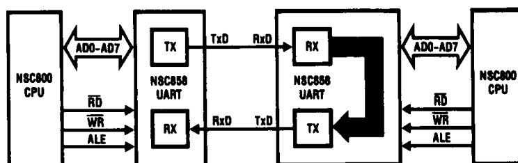
FIGURE 5. Remote Loopback
