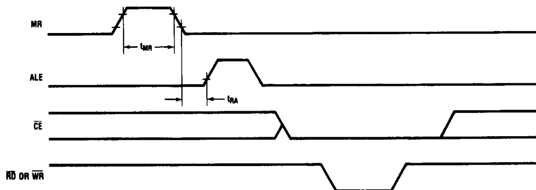
Reset Timing
