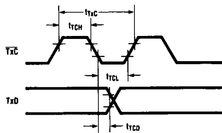
Transmitter Timing
