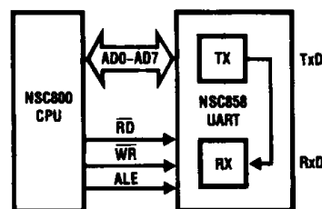
FIGURE 4. Local Loopback
