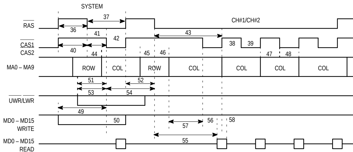
Figure 11-6. DRAM Timing
