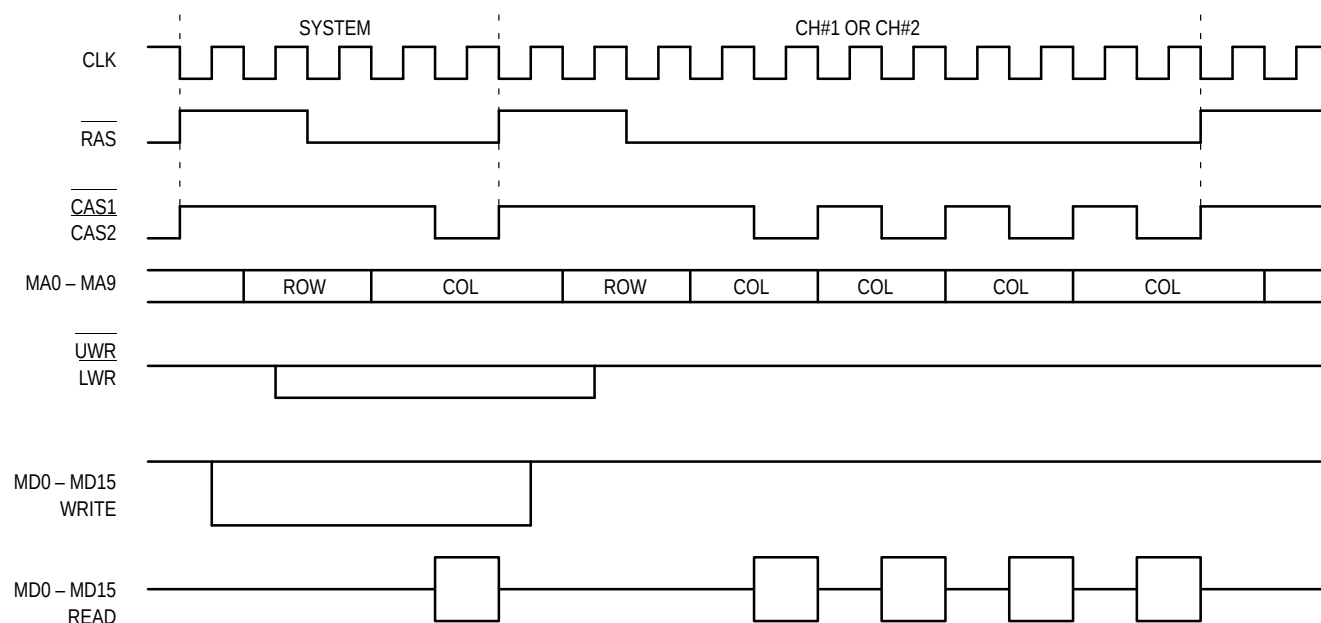
Figure 4–3. DRAM Timing
