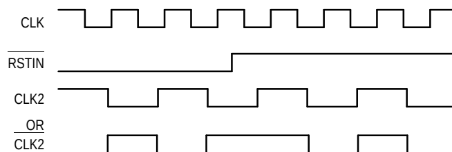
Figure 3–2. CLK2 Clocking and Resetting
