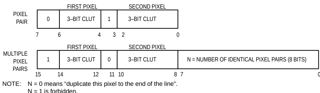
Figure 6-4. Run-length Format in 3 Bits/Pixel
