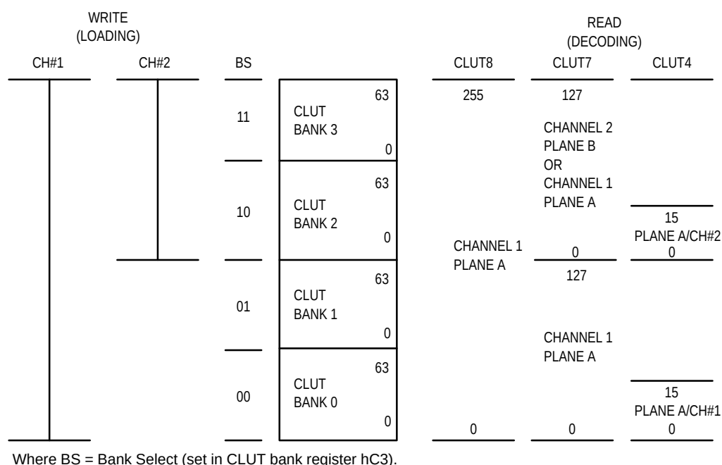
Figure 7–2. CLUT Organization
