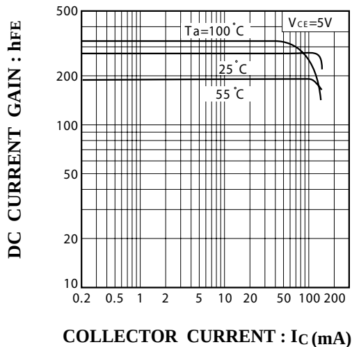
Fig.5 DC current gain vs. collector current (11)
