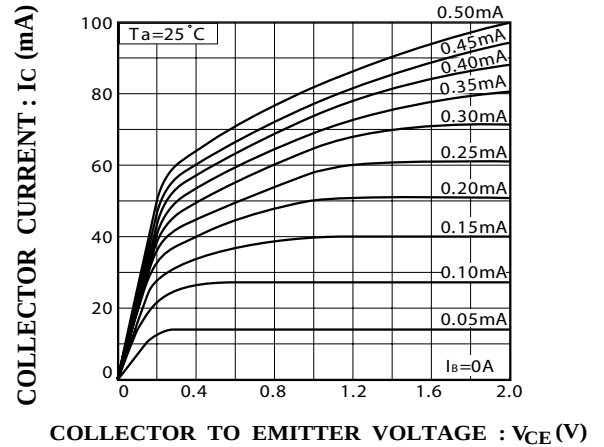
Fig.2 Grounded emitter output characteristics (1)
