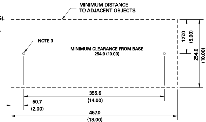
MOUNTING DETAIL
