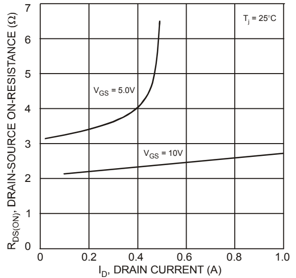
Fig. 9 On-Resistance vs. Drain Current (2N7002)
