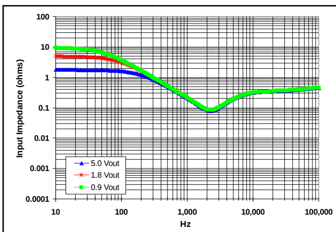
Figure 20: Magnitude of incremental input impedance ( Z_{in} = v_{in}/i_{in} ) for nominal input voltage at full rated power.
