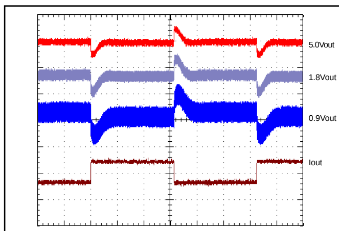
Figure 12: Output voltage response for 0.9V, 1.8V, 5V units to step-change in load current (50-75-50% of I_{out} max; di/dt=3A/\mu s ). Load cap: 470 \mu F, 100m \Omega ESR tant, 10 \mu F cer. Ch 1: I_{out} (10A/div), Ch 2-4: Vout (100mV/div).
