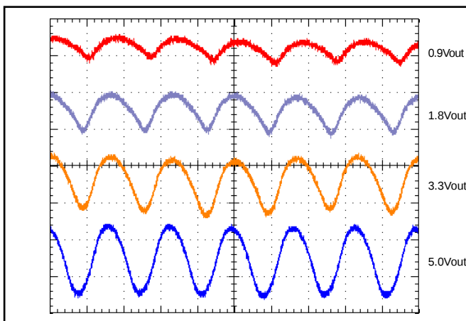
Figure 16: Output Voltage Ripple at nominal input voltage and rated load current (50 mV/div). Load capacitance: 22\ \mu\text{F} ceramic cap. Bandwidth: 20 MHz. See Figure 13.
