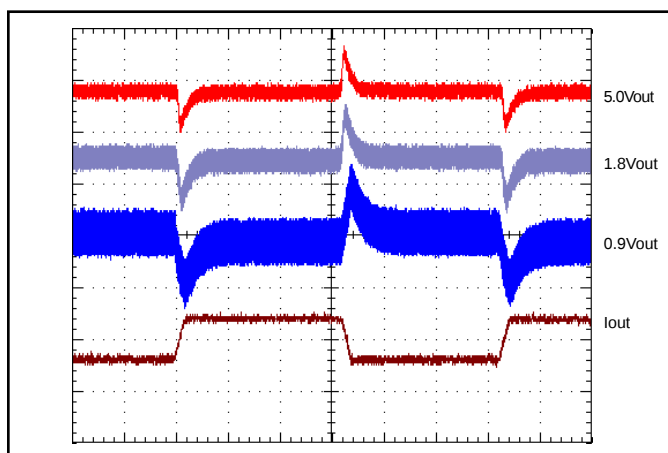
Figure 11: Output voltage response for 0.9V, 1.8V, 5V units to step-change in load current (50-75-50% of I_{out} max; di/dt=0.1A/\mu s ). Load cap: 100 \mu F, 100m \Omega ESR tant, 10 \mu F cer. Ch 1: I_{out} (10A/div), Ch 2-4: Vout (100mV/div).
