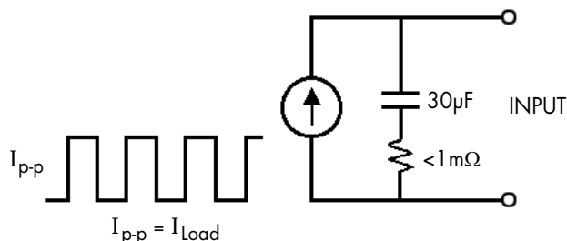
Figure E: Equivalent model for input ripple
