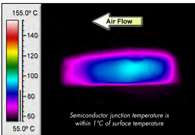
Figure 6: Thermal plot of 1.8Vo, 2.5Vo converters at nominal Vin and 16 amp load current mounted on a 70°C, 6-Layer, 2 oz. copper board (typical installation).
