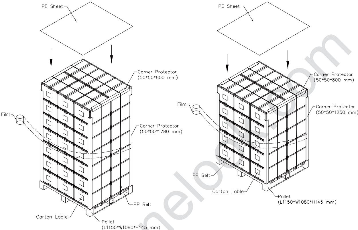
Figure. 7-3 Packing method
