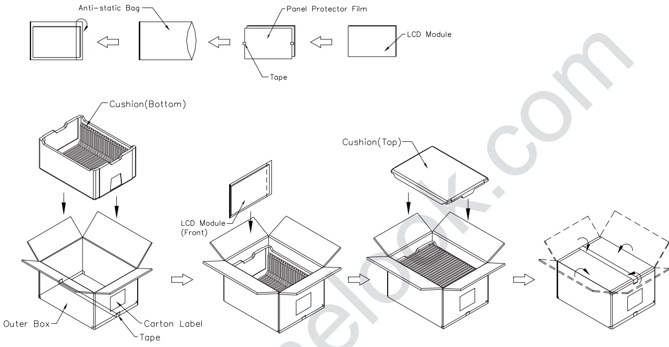
Figure. 7-2 Packing method
