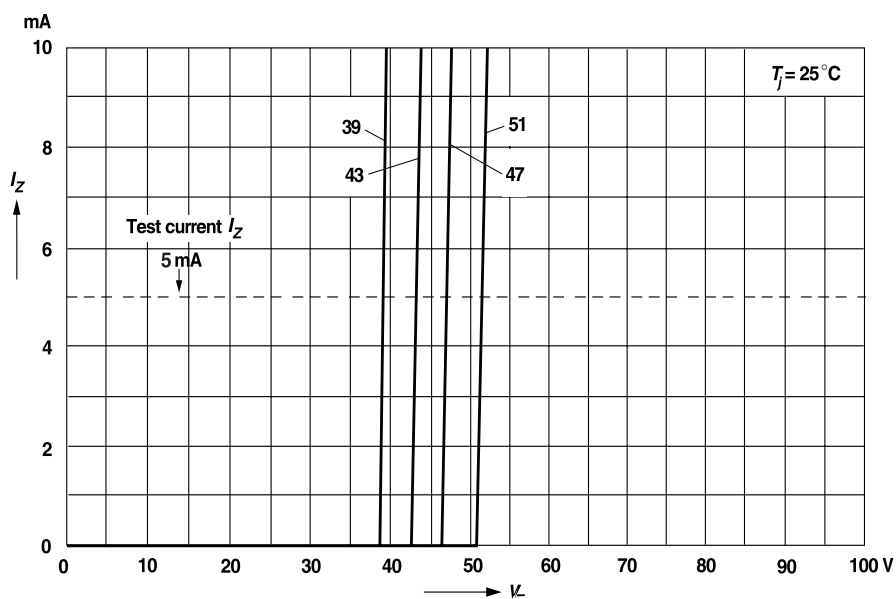
Figure 18. Breakdown Characteristics
