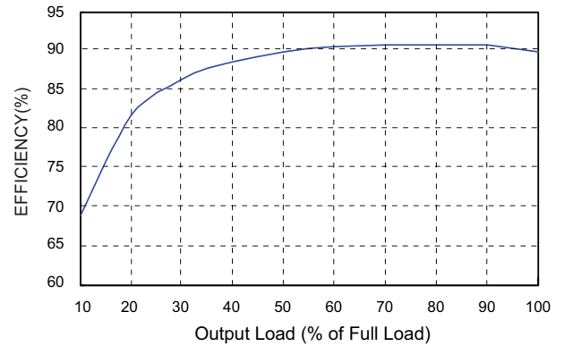
DCQEB75-48S05 Efficiency vs Output Load
