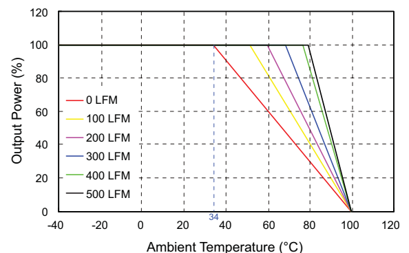
DCQEB75-48S05 Derating Curve With Heatsink 7G-0029A-F
