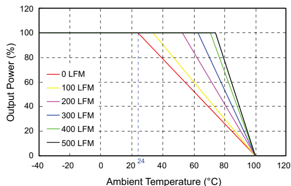
DCQEB75-48S05 Derating Curve
