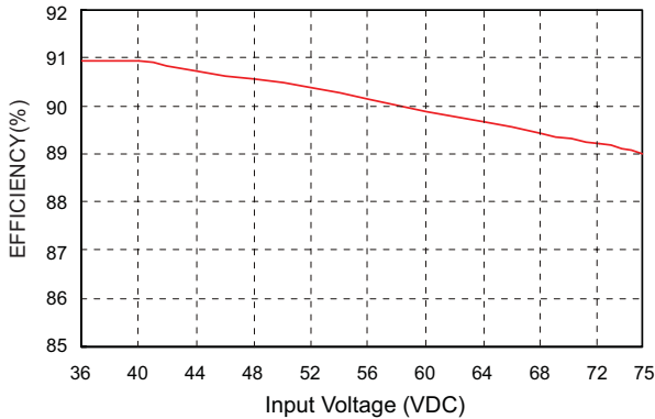
DCQEB75-48S05 Efficiency vs Input Voltage
