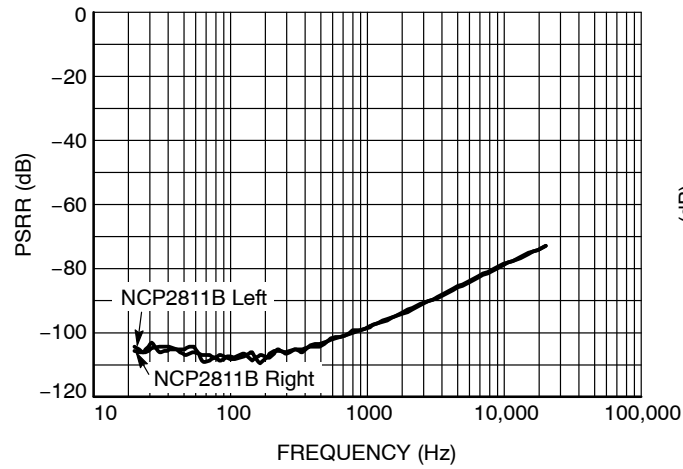
Figure 23. PSRR at V_p = 3.6\text{ V}
