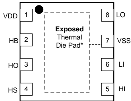
DRM Package 8-Pin SON Top View
