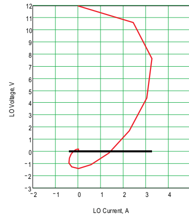
Figure 25. Turnoff Voltage and Current Switching Diagram
