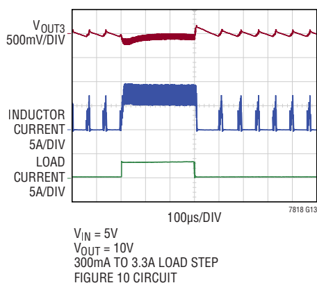
Load Step (Boost) Burst Mode Operation
