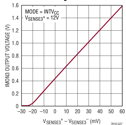
Boost Current Monitor Voltage vs Sense Voltage
