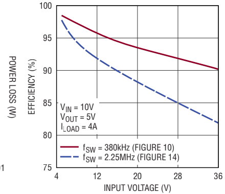
Efficiency vs Input Voltage (Buck)
