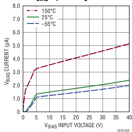
Shutdown Current vs V BIAS Input Voltage
