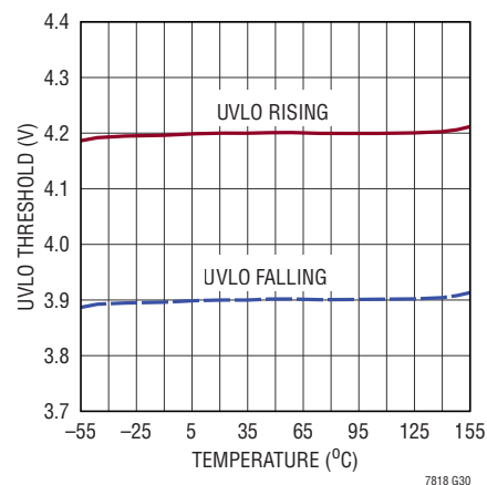
INTV CC Undervoltage Lockout Thresholds vs Temperature
