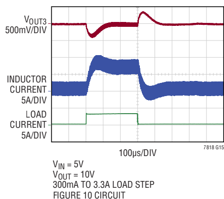
Load Step (Boost) Forced Continuous Mode
