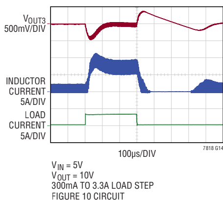
Load Step (Boost) Pulse-Skipping Mode
