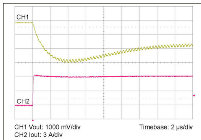
Figure 10 — 0-6.3 A load step with 100 \mu F input capacitor and no output capacitor.
