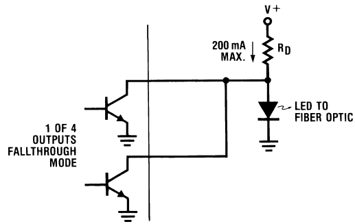
DP8311 Parallel Outputs (200 mA) Drivers*
