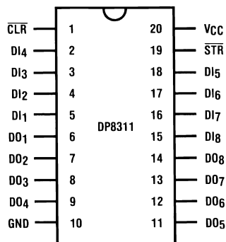
Dual-In-Line Package
